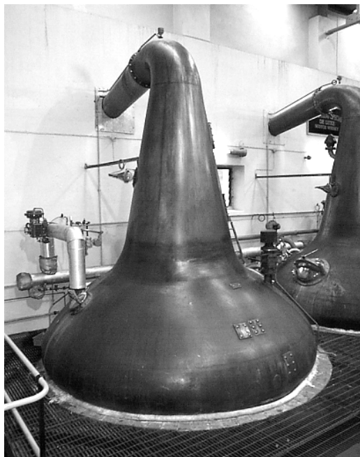
Brennblase - Longmorn
